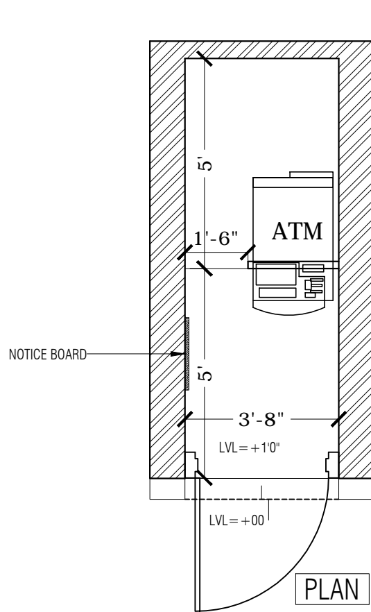
ATM PLAN, UCO BANK TILKAMANJHI = 37 SQFT
