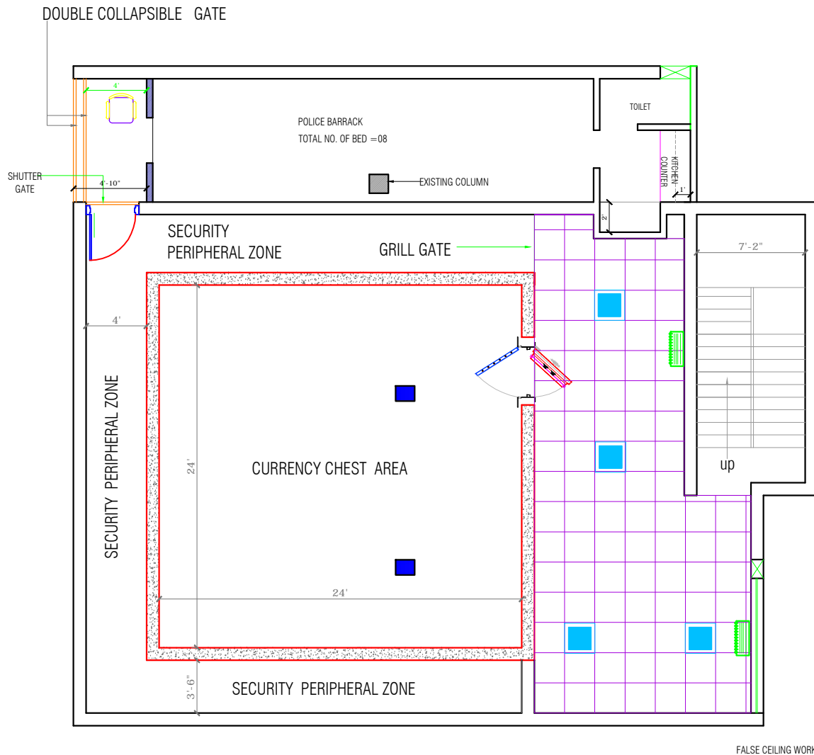
FALSE CEILING LIGHT AND AC LAYOUT PLAN CURRENCY CHEST FLOOR
